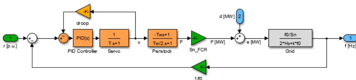
Figure 1 Simple single machine- single system model used.
