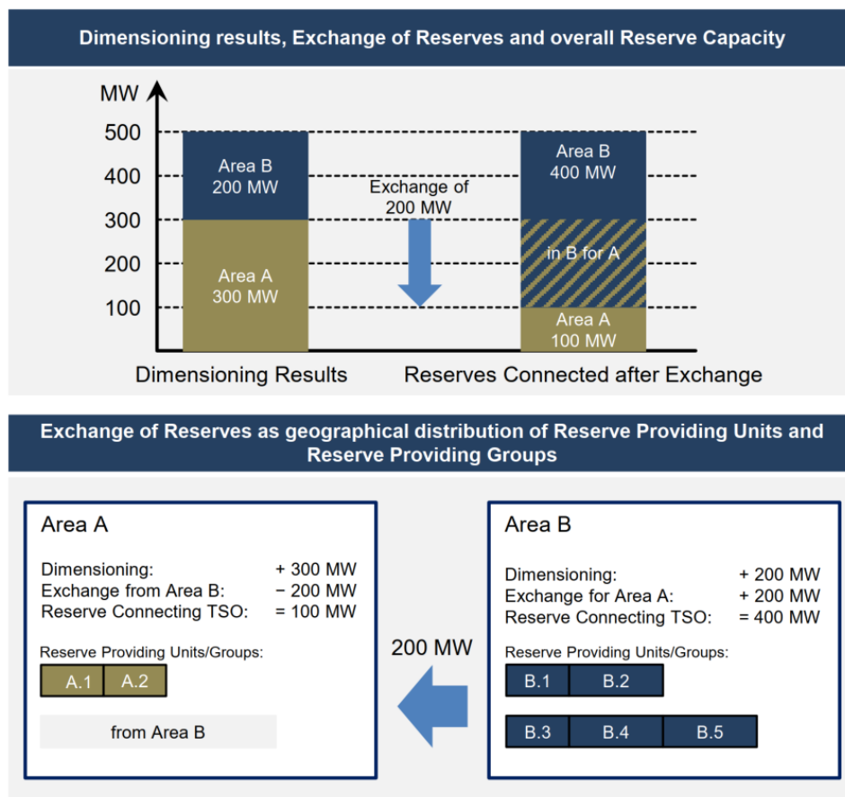
Figure 1: Exchange of reserve capacity – simple example
