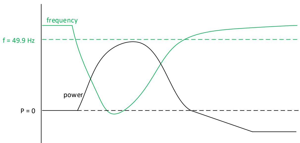
Figure 3.5 Recharging of energy storage facility in Frequency Containment Reserve for Disturbances
