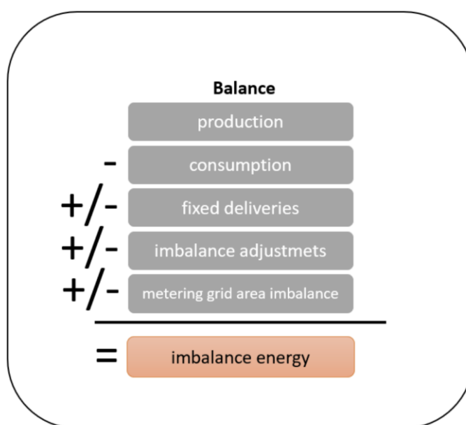
Figure 1. Imbalance calculation
