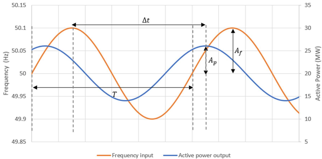
Figure 2: FCR-N sine response testing.
